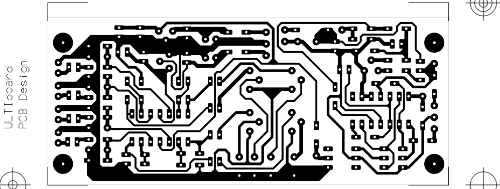
CAR_PRE, Bottom (Aug. 03, 2005) (15:06) (PCB) SCALE: 100% REFLECTED Drill Ref Pnt: 4.875, 0.000 (inch)
