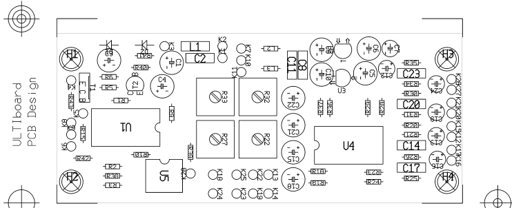
CAR_PRE, Silkscreen (Aug. 03, 2005) (15:06) (PCB) SCALE: 100% Drill Ref Pnt: 0.000, 0.000 (inch)
