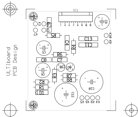
TDA7294, Silkscreen (Aug. 03, 2005) (16:34) (PCB) SCALE: 100% Drill Ref Pnt: 0.451, 0.000 (inch)
