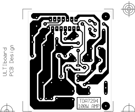
TDA7294, Bottom (Aug. 03, 2005) (16:39) (PCB) SCALE: 100% REFLECTED Drill Ref Pnt: 2.725, 0.000 (inch)
